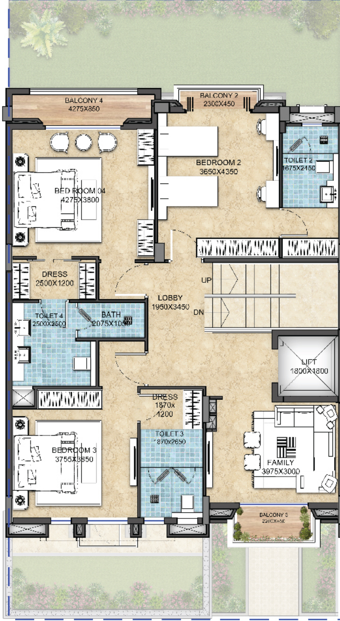
First Floor
